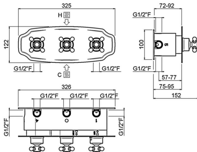
Art. 21345/O-CR; Art. 21355/O-CR; Art. 21365/O-CR; Art. 21345-CR; Art. 21355-CR; Art. 21365-CR
